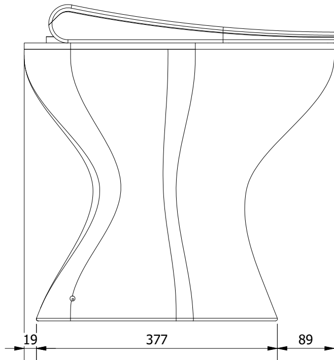
SIDE VIEW
